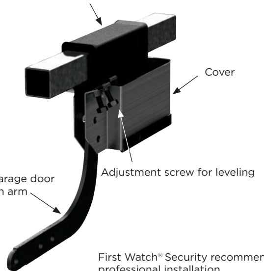
Existing garage door carriage
